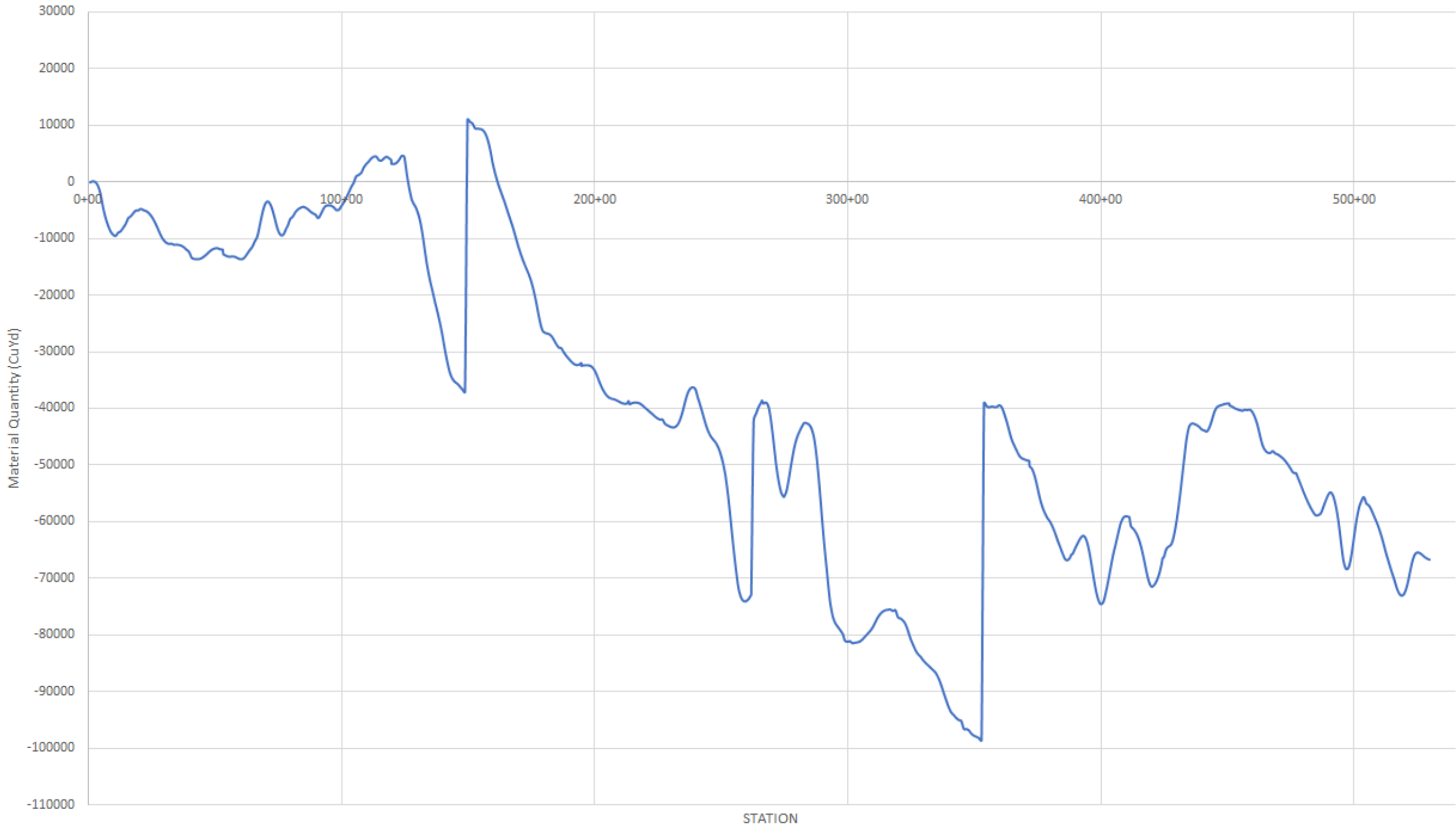
Mass Haul Diagram - 04EW
