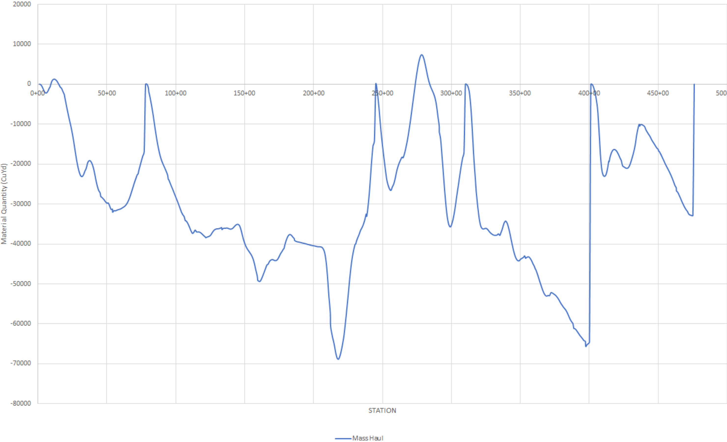
Mass Haul Diagram - 069D
