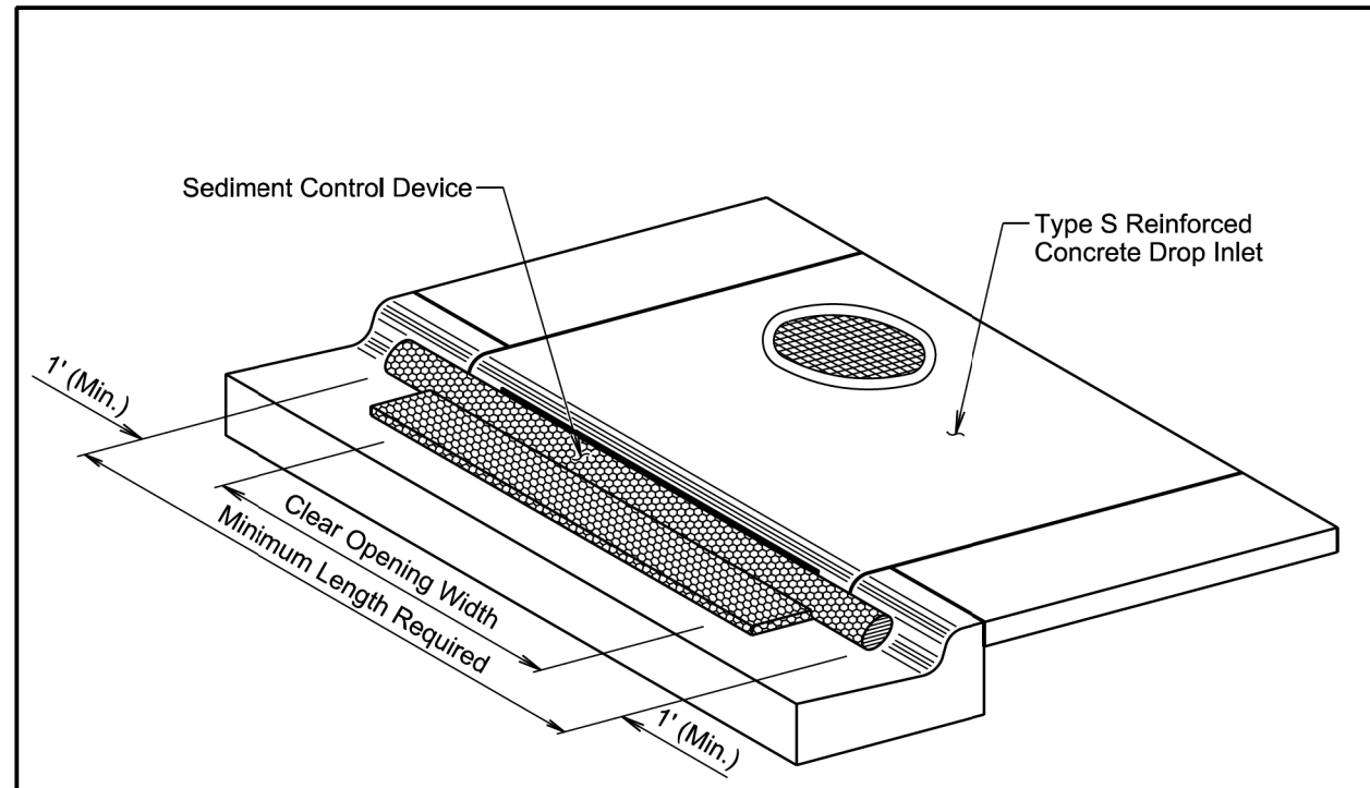
ISOMETRIC VIEW
