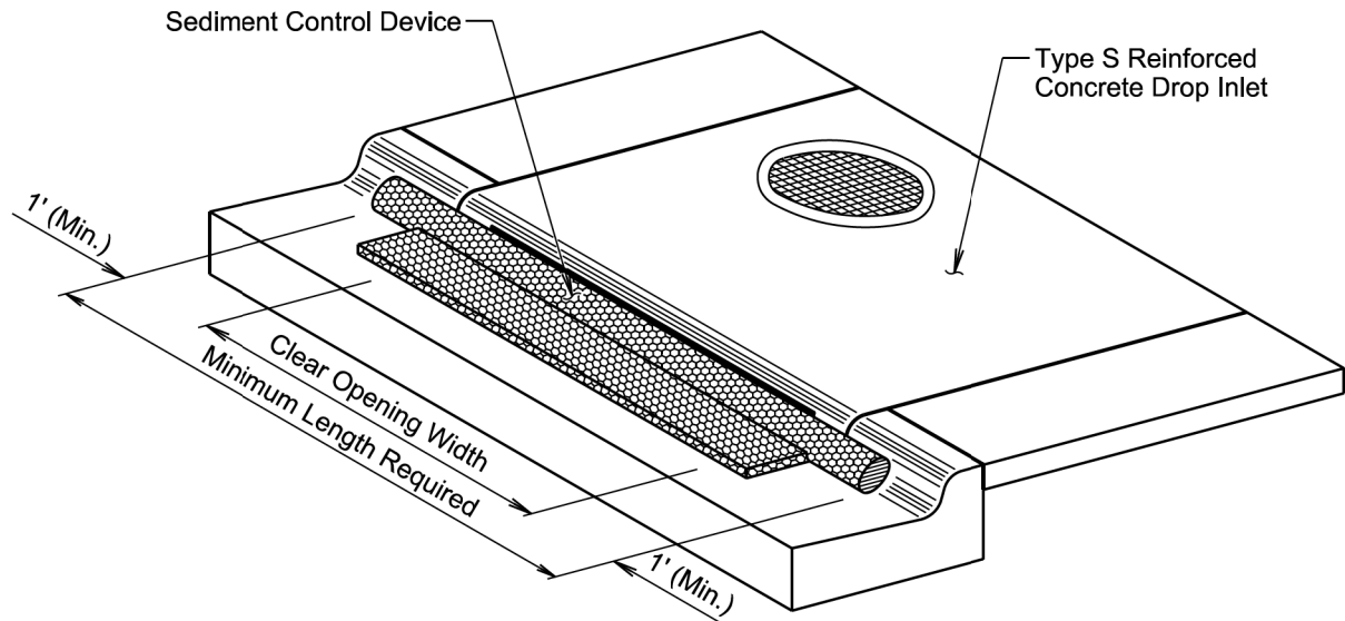
ISOMETRIC VIEW
