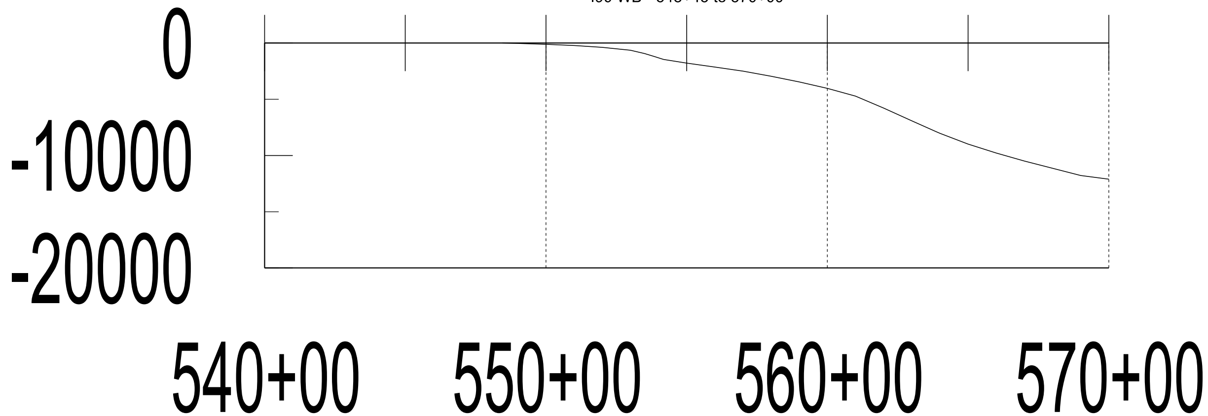
Mass Haul Diagram 190 WB - 548+45 to 570+00
