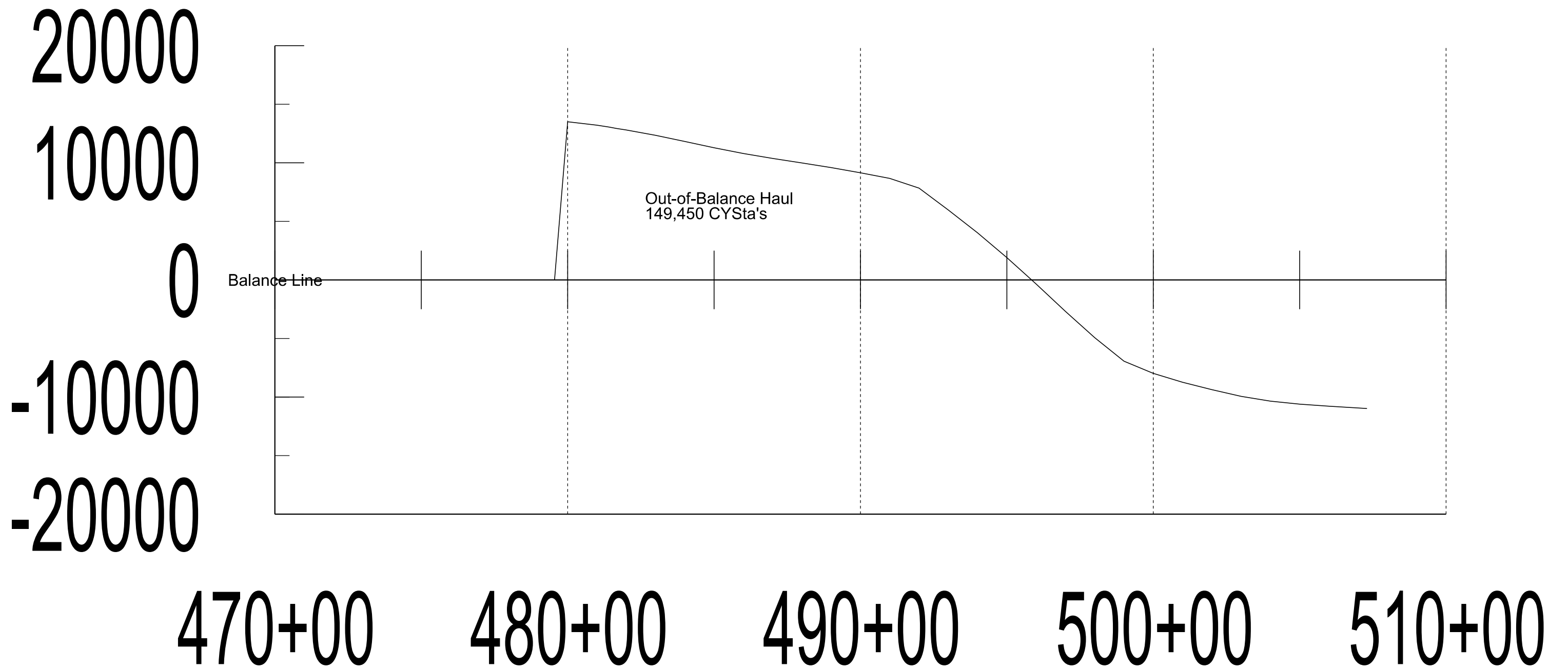
Mass Haul Diagram for I90 WB - 479+55 to 507+30
