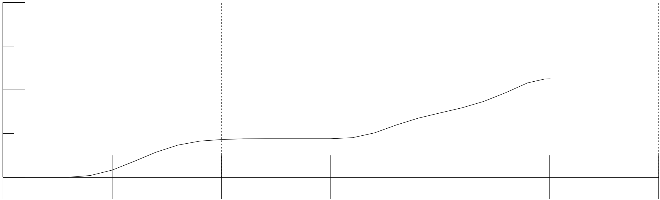
Mass Haul Diagram for Exit 350-Ramp C Ditch
