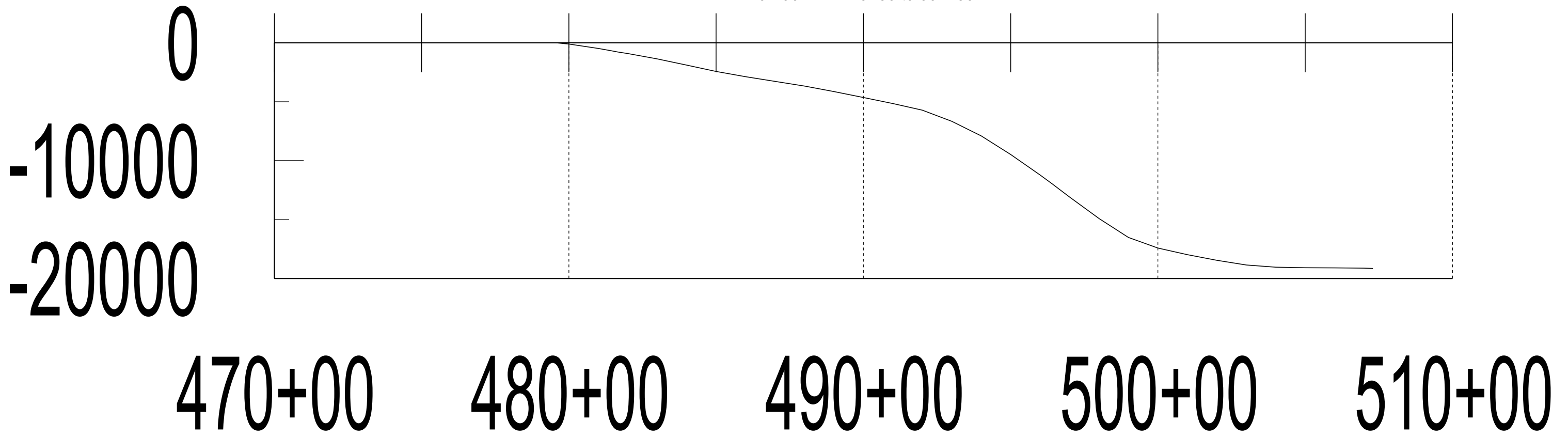
Mass Haul Diagram for I90 EB - 479+55 to 507+30
