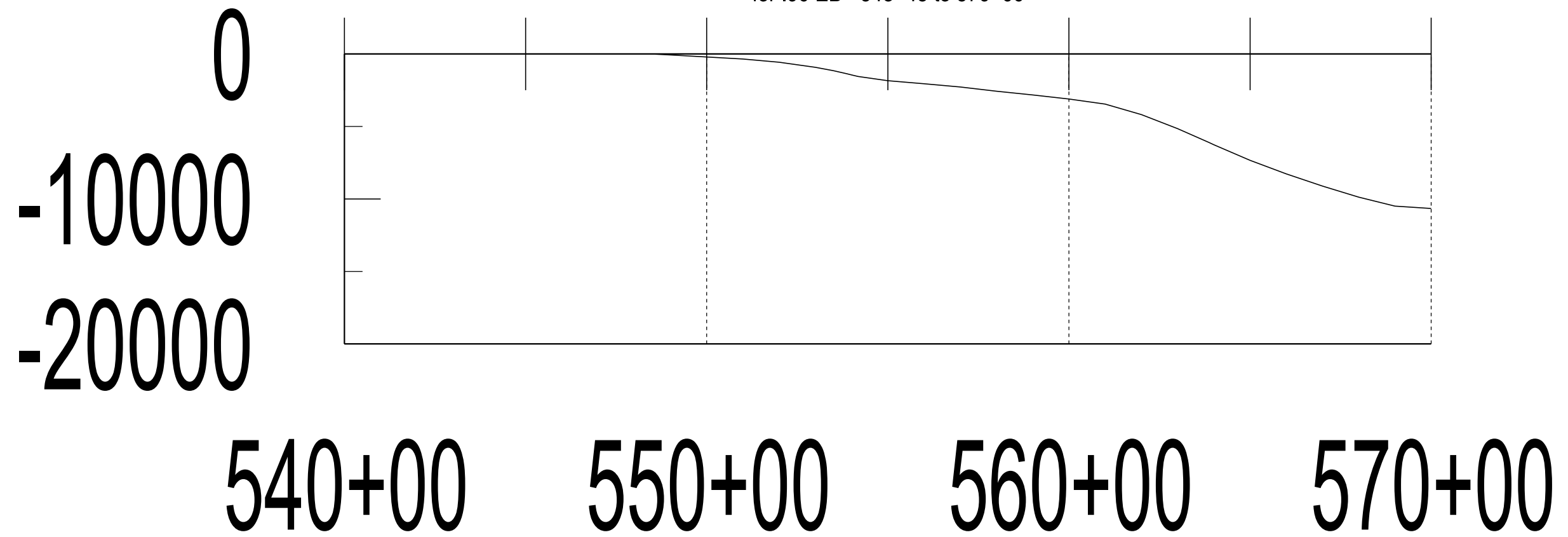
Mass Haul Diagram for I90 EB - 548+45 to 570+00
