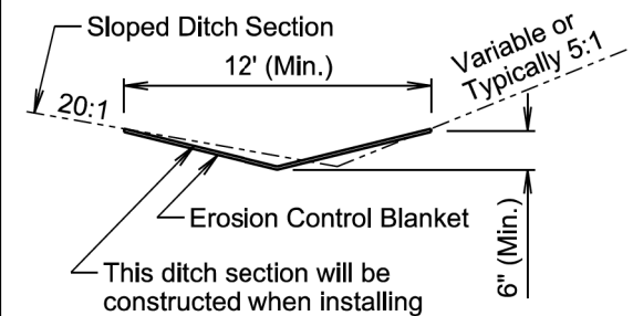
SLOPED DITCH SECTION
