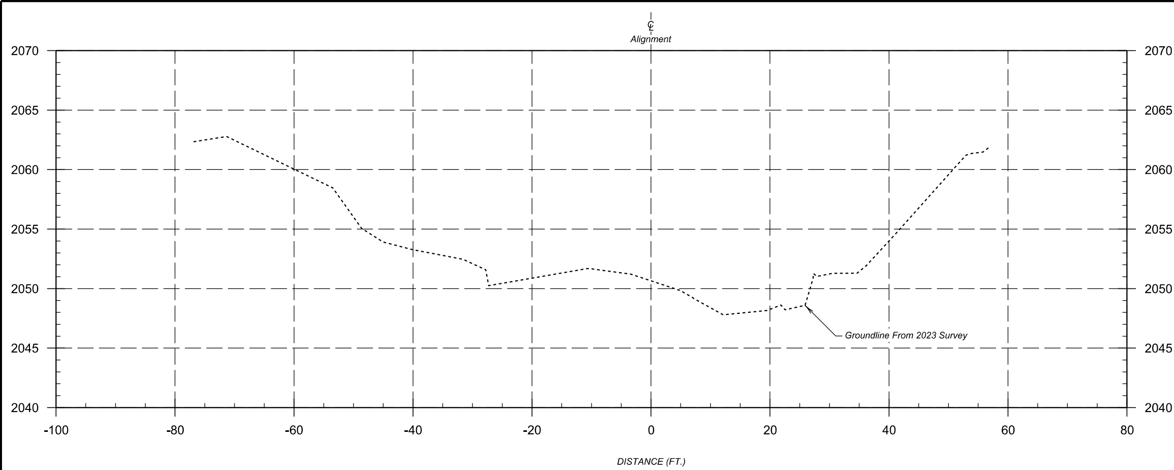
MAINLINE CROSS SECTION 0+50
