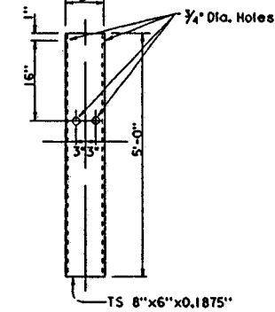
STEEL TUBE ANCHOR
