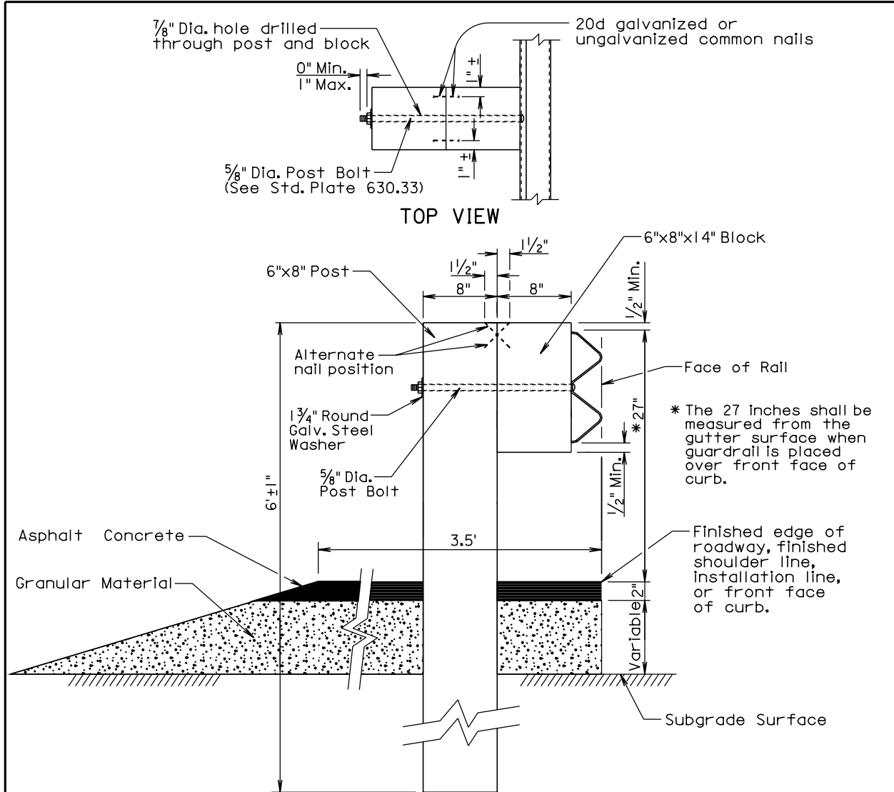
TRANSVERSE SECTION
