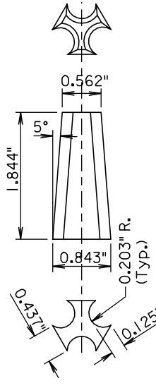
DETAIL G (TYPICAL WEDGE FOR ALL SPLICES AND CABLE FITTINGS)
