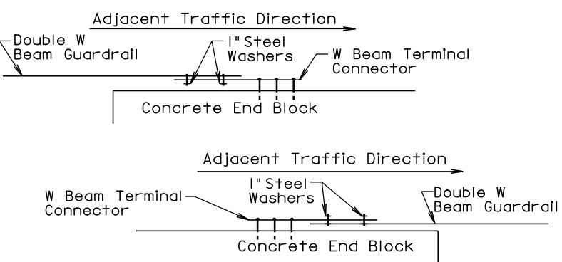
ELEVATION W BEAM TERMINAL CONNECTOR
