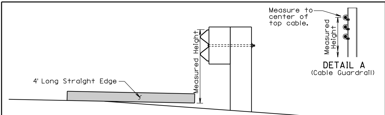
ELEVATION VIEW (Guardrail Adjacent to Differential Slopes)
