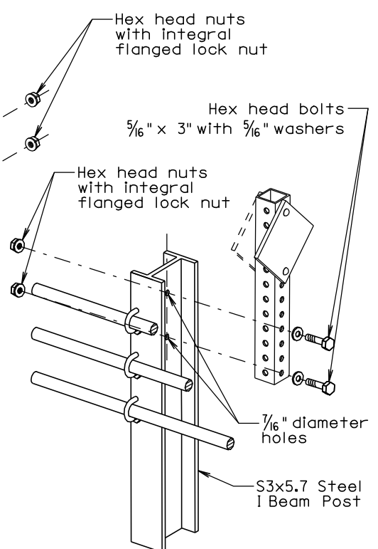
△ C 3 CABLE GUARDRAIL DELINEATION ( 4" x 4" Delineator on I Beam Steel Post )
