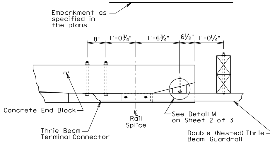
DETAIL J
