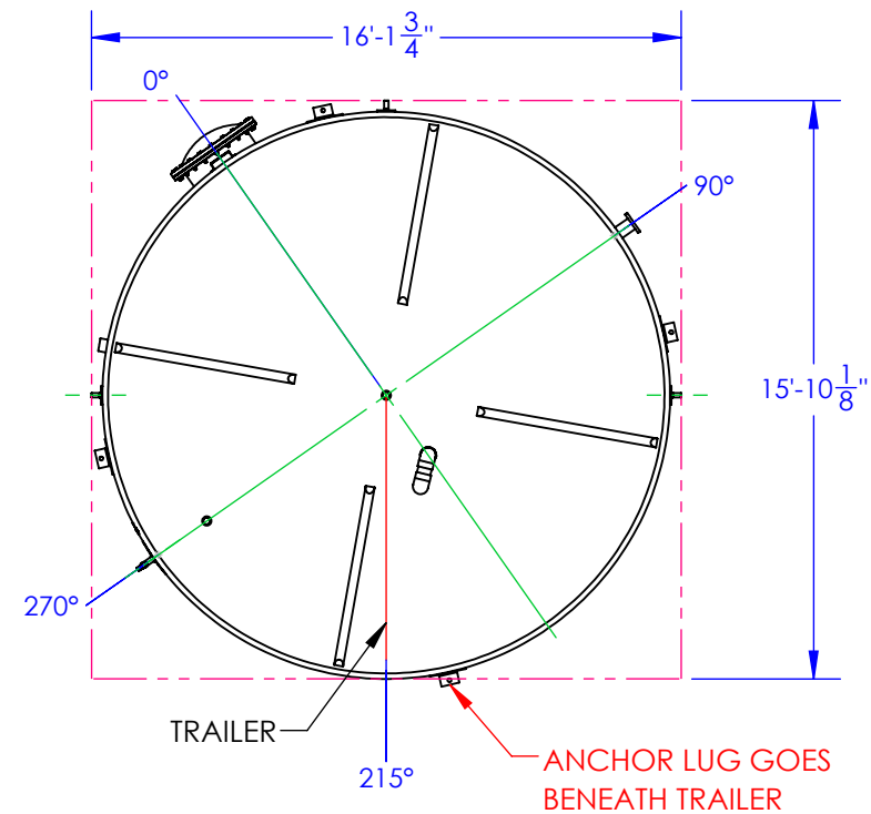
SHIPPING ENVELOPE DETAIL
