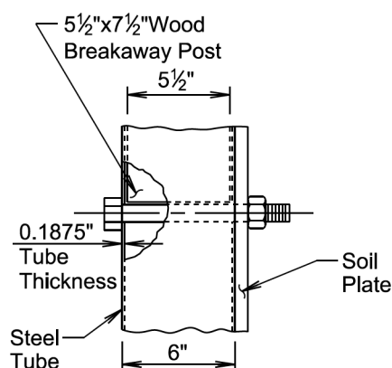
DETAIL D
