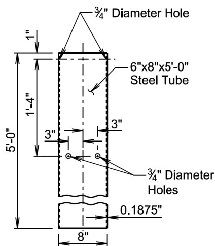
STEEL TUBE
