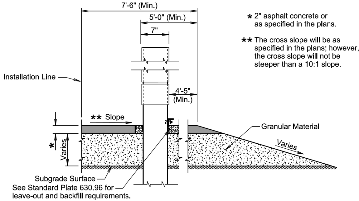
TRANSVERSE SECTION (SoftStop MGS MASH Tangent End Terminal Shown)
