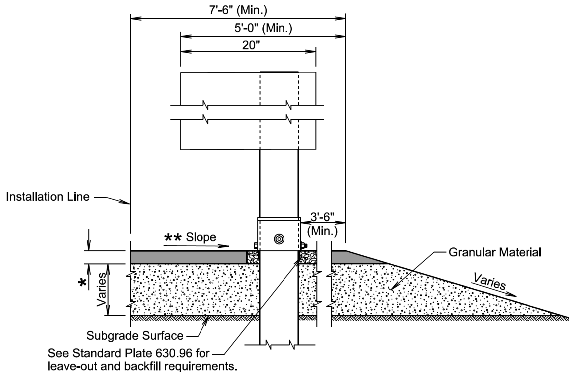
TRANSVERSE SECTION (MSKT-SP-MGS MASH Tangent End Terminal Shown)
