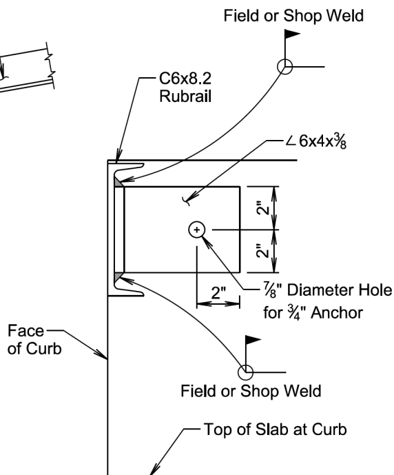
VIEW H-H (Anchor and Rail Not Shown) (For Bridge Rail Class B Design 1T or 2T)
