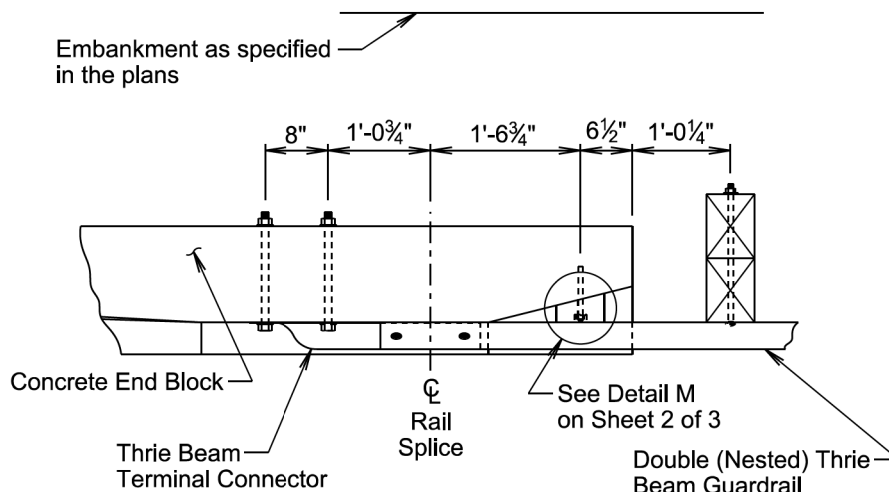
DETAIL J
