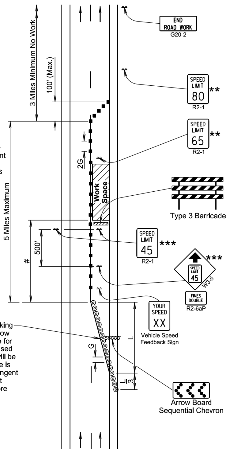
DETAIL A
