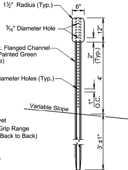
ELEVATION VIEW
