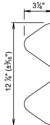
VIEW B-B
