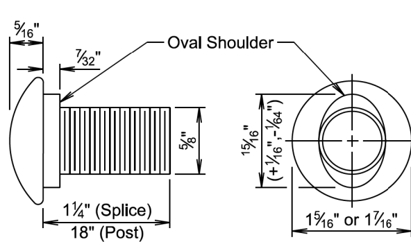
SPLICE BOLT AND POST BOLT (5/8" Button Head Bolt)
