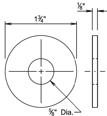
WASHER (The washer will be placed between the back side of wood post and the recess nut, see sheet 1 and 2.)
