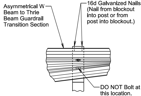
DETAIL L
