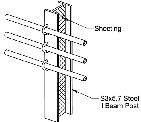
△ 3 CABLE GUARDRAIL (LOW TENSION) DELINEATION
