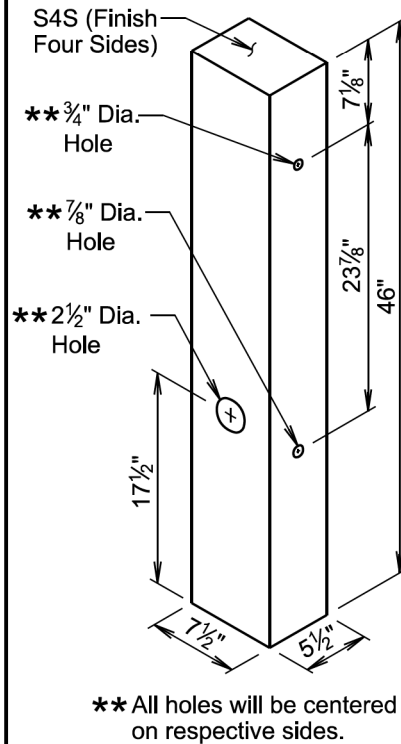
WOOD BREAKAWAY POST
