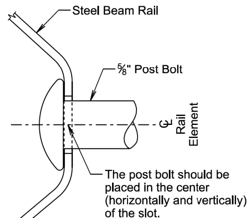
SECTION VIEW (At Post Bolt)
