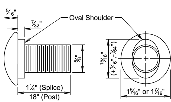
SPLICE BOLT AND POST BOLT (5/8" Button Head Bolt)
