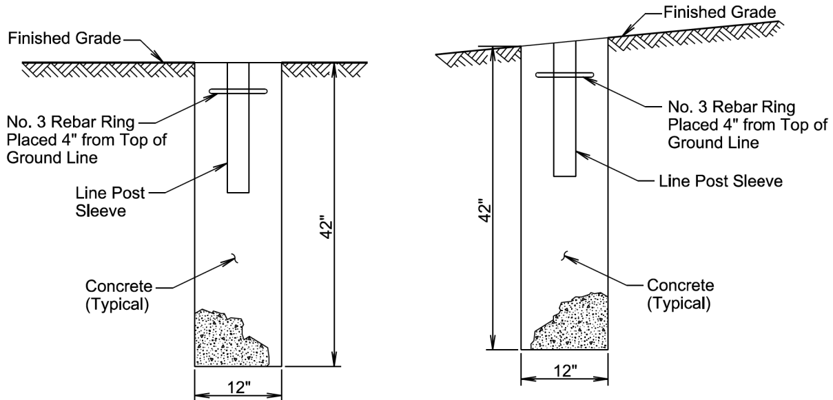
Line Post Concrete Footing on Slopes 10:1 or Flatter
