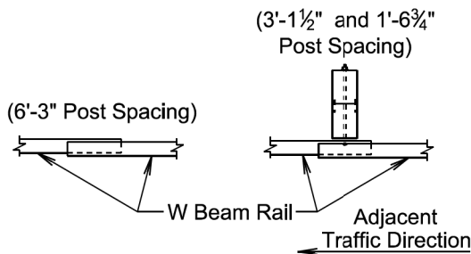
PLAN VIEW (Lap Splice) (Lap rail in direction of adjacent traffic.) (8 splice bolts and 8 recess nuts per splice, NO washers)
