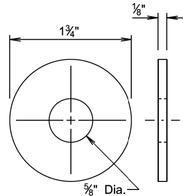
WASHER (The washer will be placed between the back side of wood post and the recess nut, see sheet 2 and 3.)
