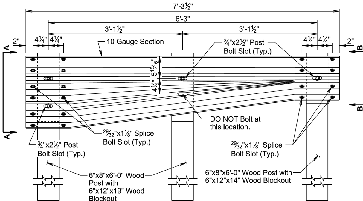
ELEVATION VIEW
