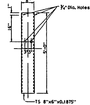
STEEL TUBE ANCHOR
