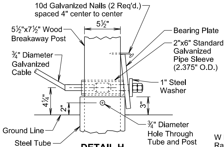
DETAIL H
