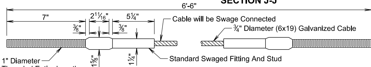
CABLE ASSEMBLY
