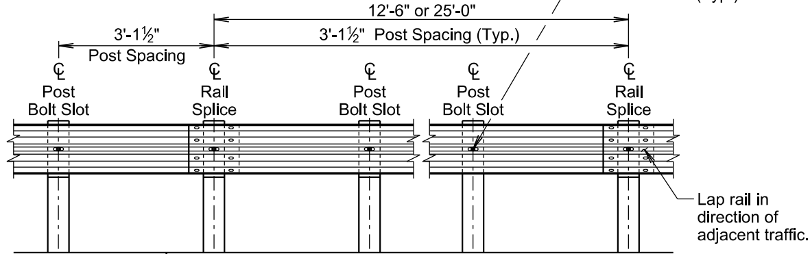
ELEVATION VIEW (3'-1 1/2" Post Spacing) Finished Surface or Ground Line The post bolt should be placed in the center (horizontally and vertically) of the slot. (Typ.)
