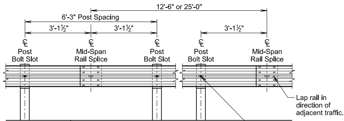
ELEVATION VIEW (6'-3" Post Spacing) Finished Surface or Ground Line The post bolt should be placed in the center (horizontally and vertically) of the slot. (Typ.)
