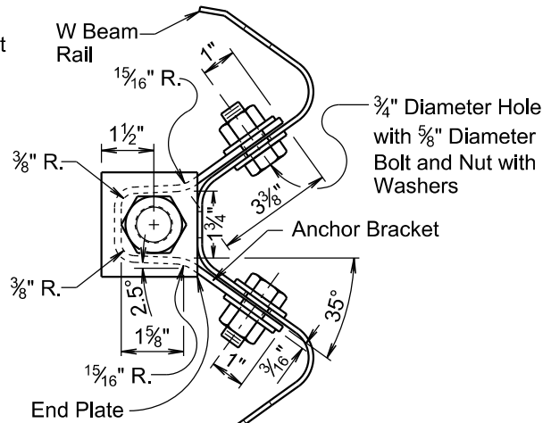
SECTION J-J
