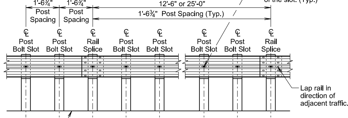
ELEVATION VIEW (1'-6 3/4" Post Spacing) Finished Surface or Ground Line The post bolt should be placed in the center (horizontally and vertically) of the slot. (Typ.)
