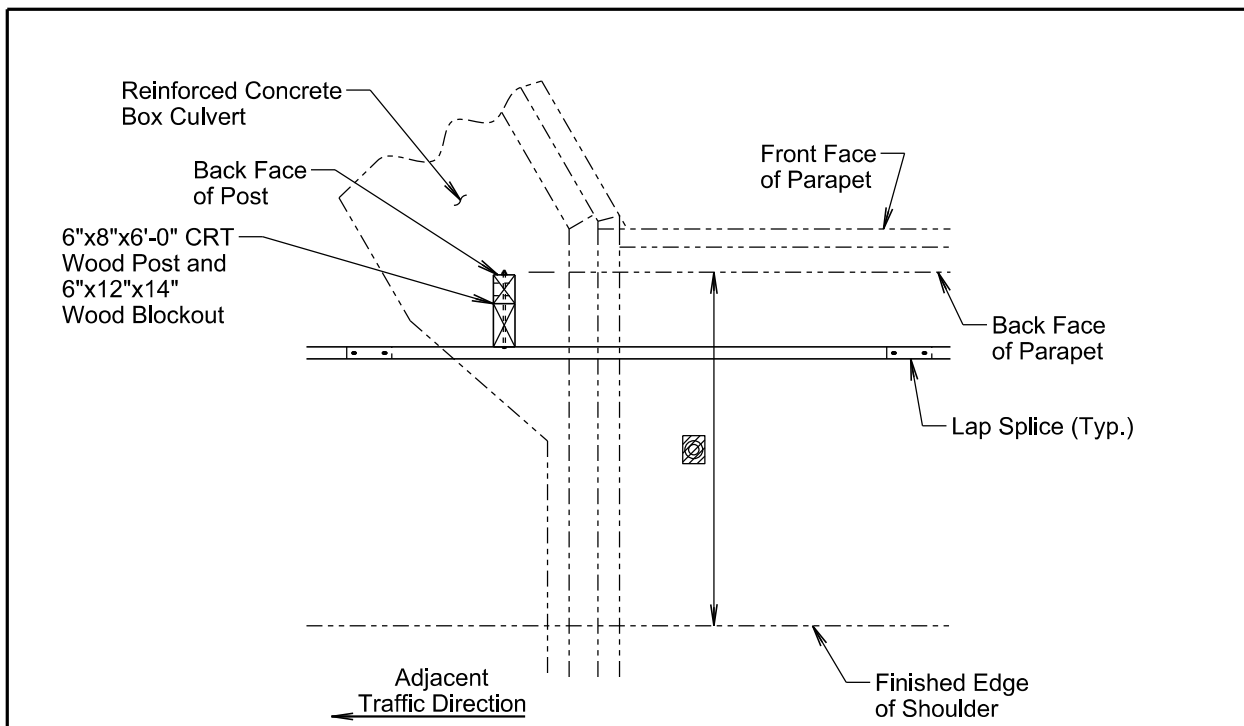
DETAIL C
