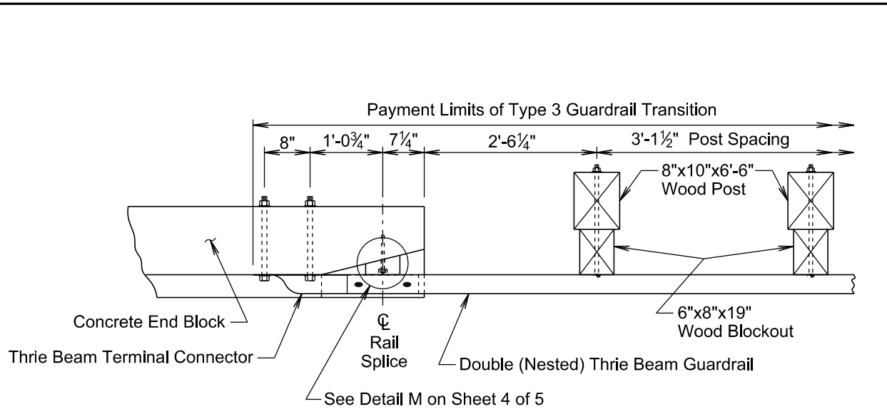
DETAIL F
