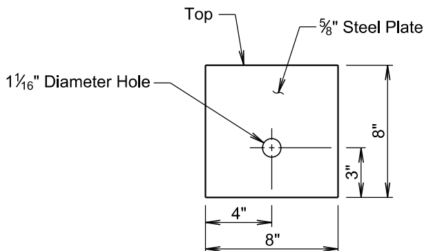
BEARING PLATE
