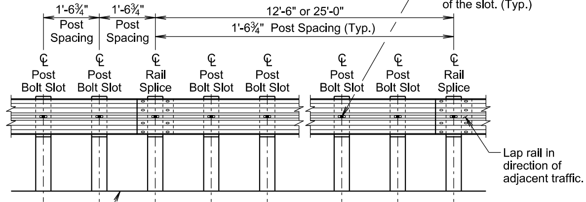
ELEVATION VIEW (1'-6 3/4" Post Spacing)
