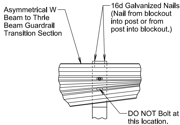
DETAIL L
