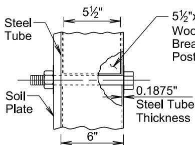
DETAIL K
