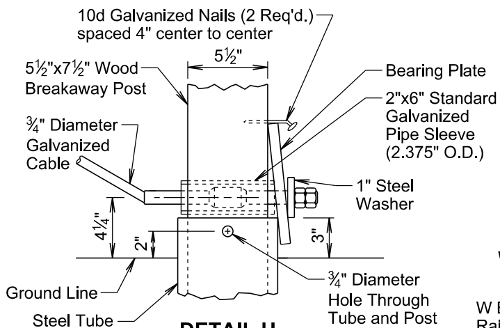
DETAIL H
