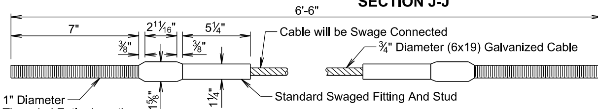
CABLE ASSEMBLY
