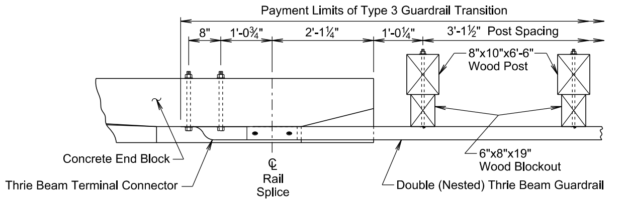
DETAIL G
