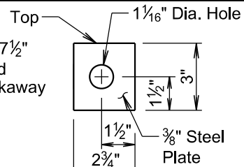
END PLATE FOR ANCHOR BRACKET
