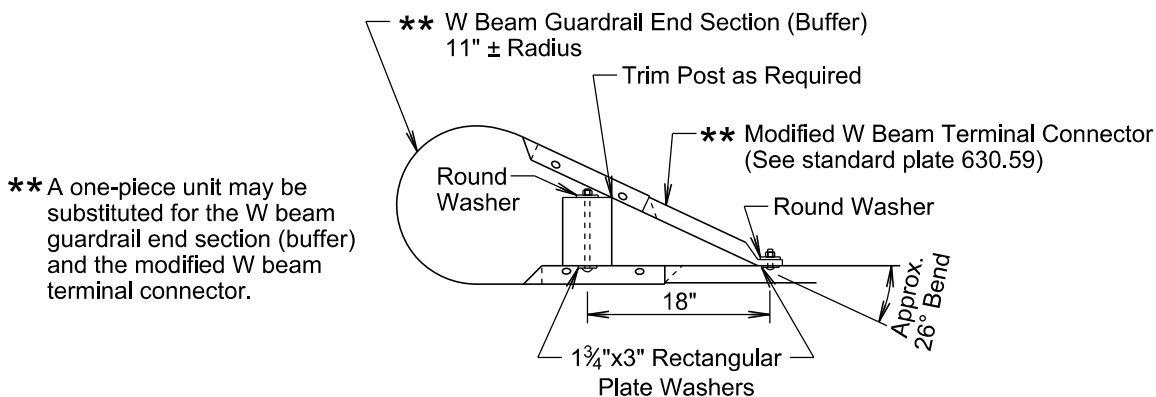
VIEW B-B
