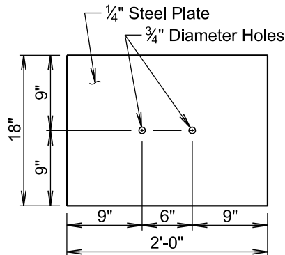
SOIL PLATE
