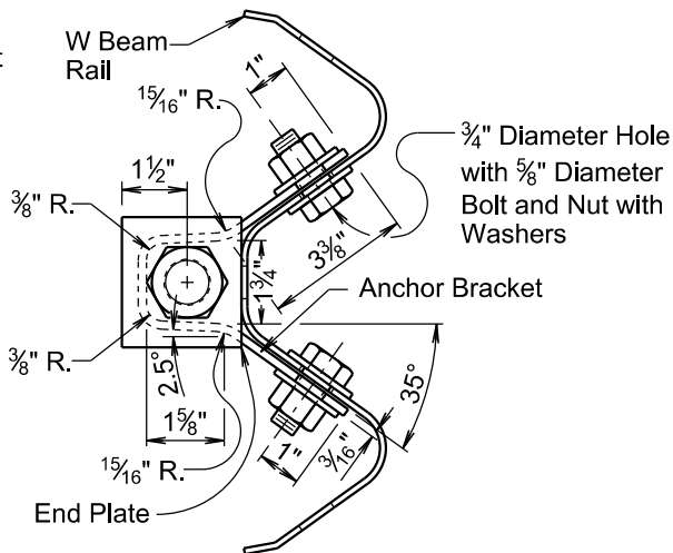
SECTION J-J
